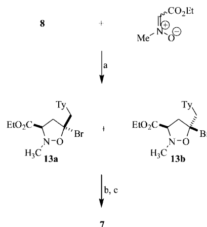
Scheme 3. a) THF, microwave at 300 W, 80 °C, 3 h; b) NaBH 4 , MeOH; c) Et 3 N.
