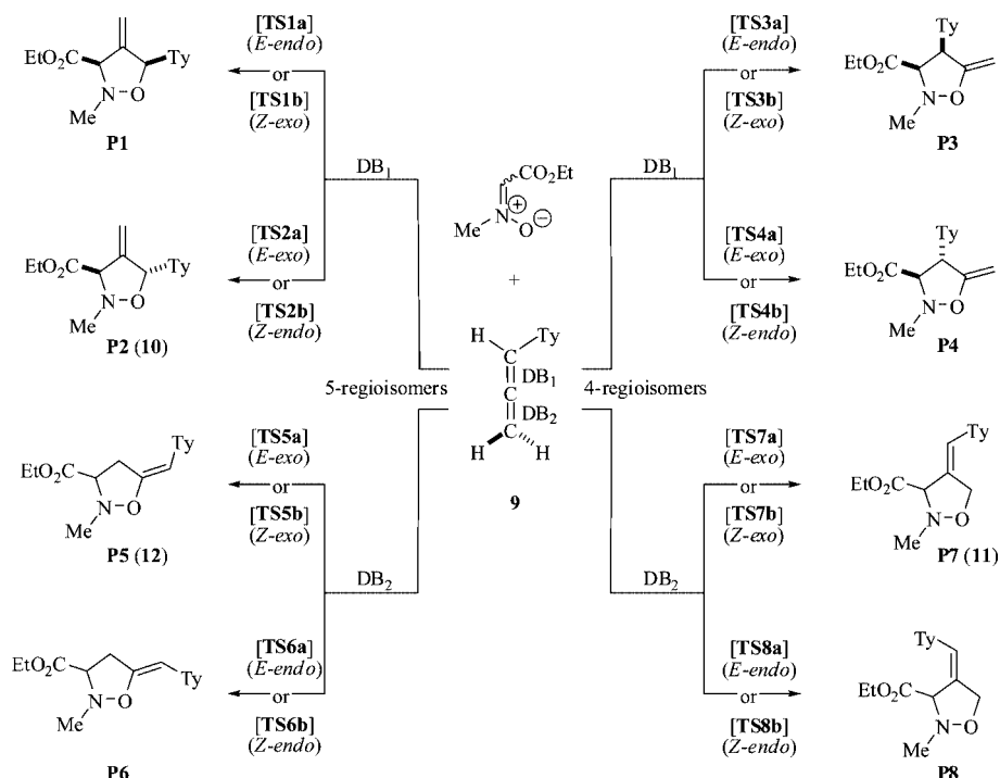
Scheme 2. Combinations of all possible transition states involved in cycloaddition.
