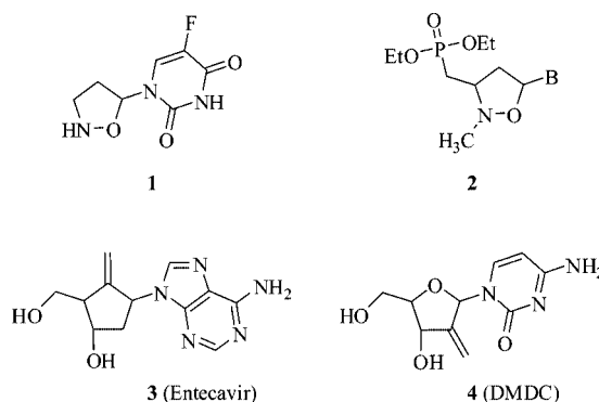
Figure 1. Nucleoside analogues.
