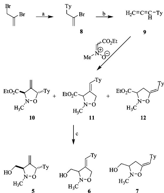
Scheme 1. a) Silylated thymine, TMSTf, CH 3 CN; b) NaOH, dioxane/H 2 O; c) NaBH 4 , dioxane, H 2 O.
